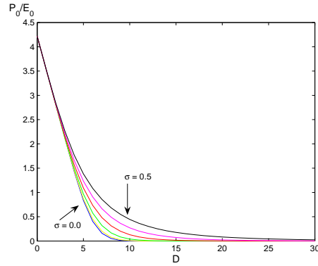
(b) PE Ratios for a 'value' firm: Expected Growth of Earnings, g = 0 .
